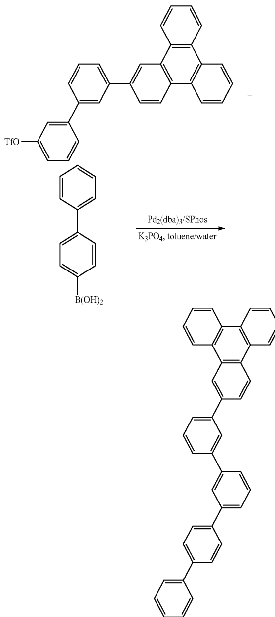
Compound 11
