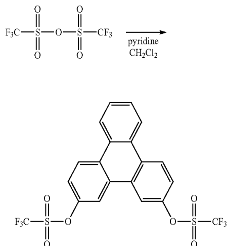
Triphenylene-2,11-dilyl bis(trifluoromethanesulfonate)
